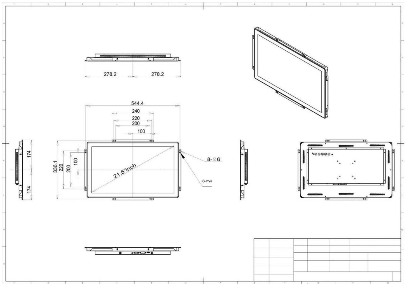
Figure 1074: Technical Drawing
