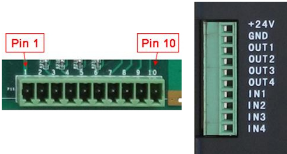
Figure 731: GPIO Connector
