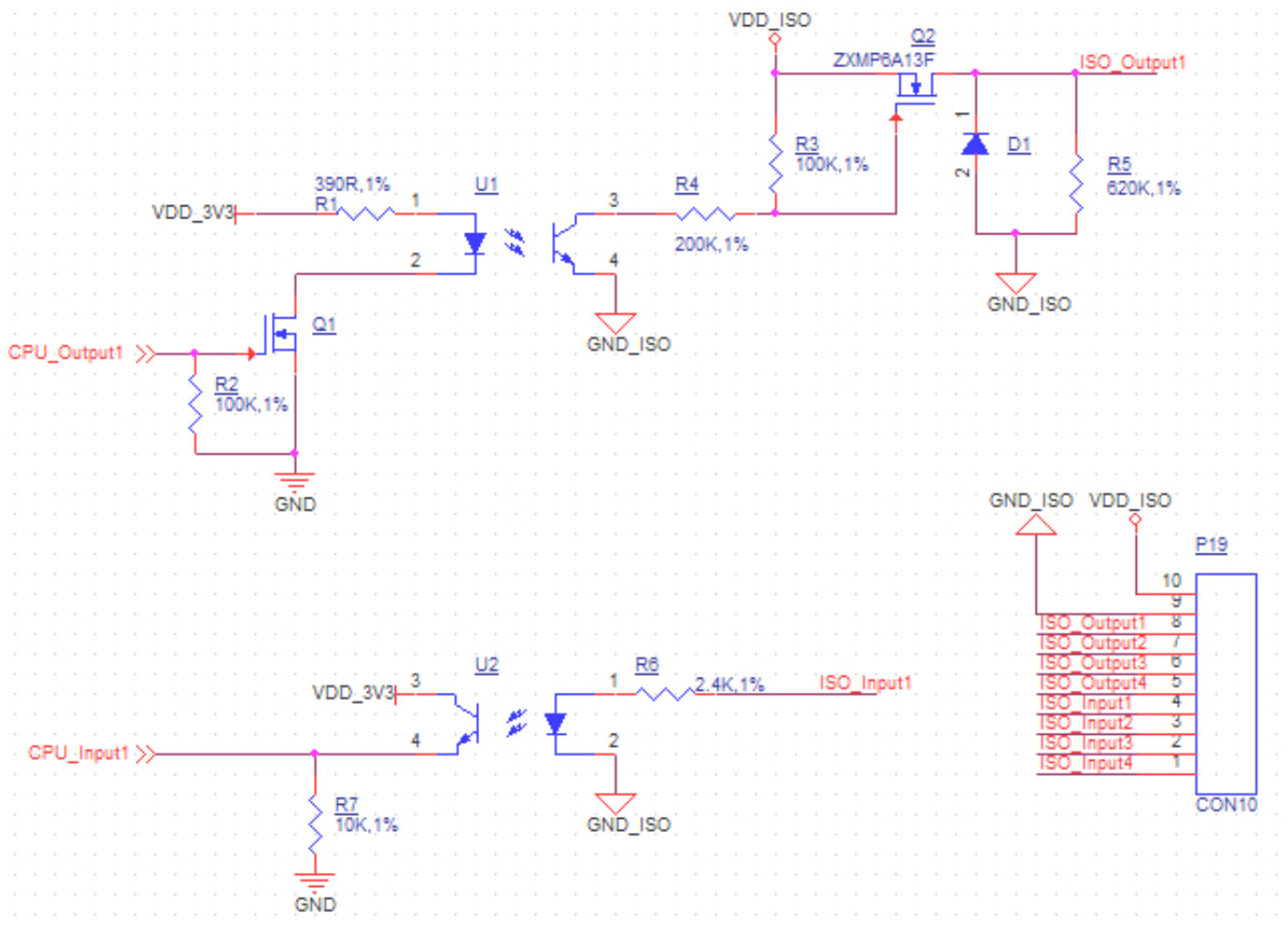
Figure 731: GPIO Connector
