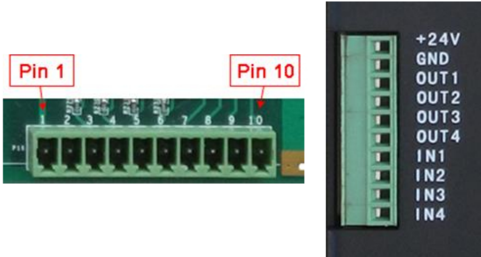
Figure 759: GPIO Connector
