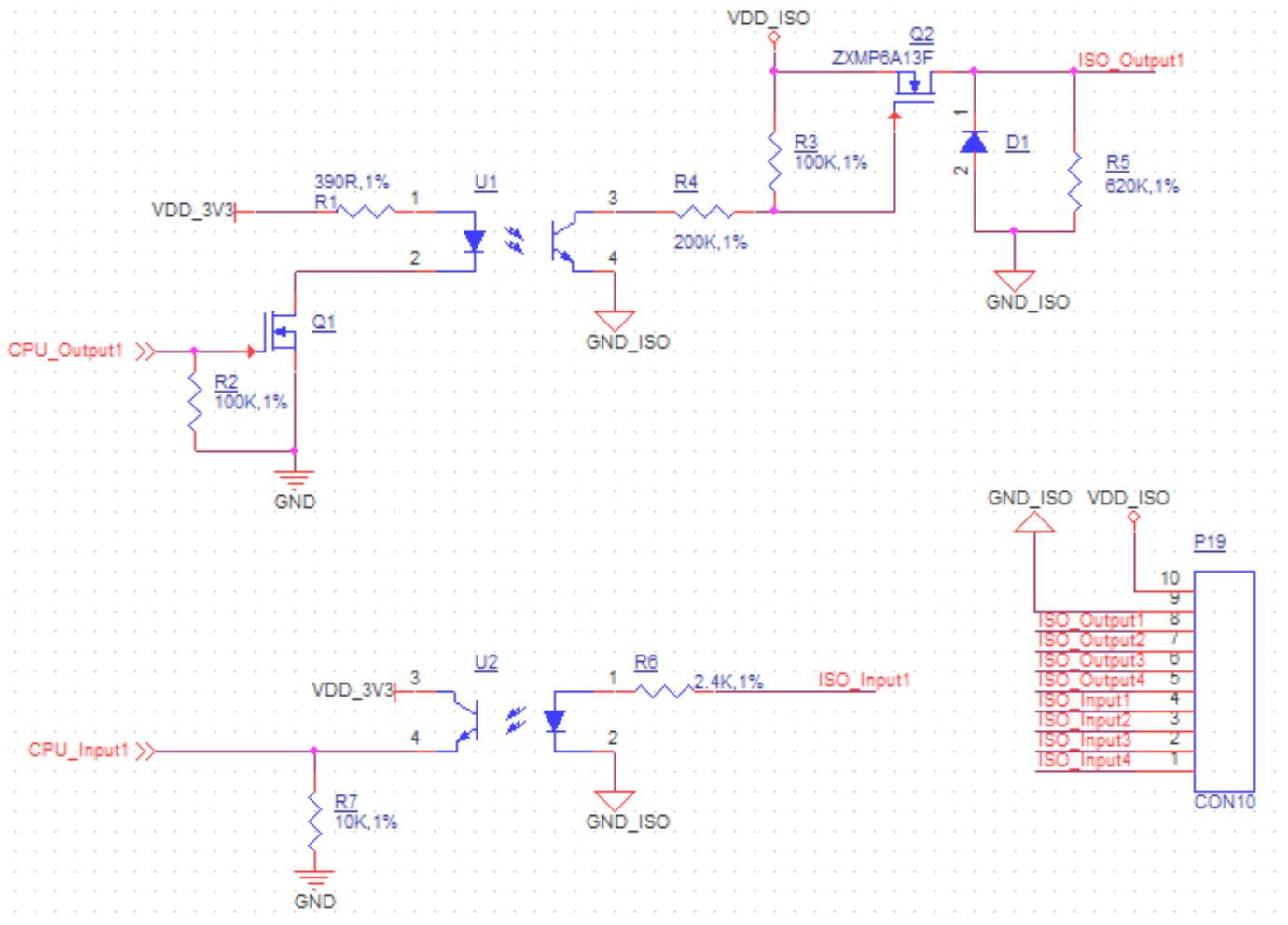
Figure 759: GPIO Connector
