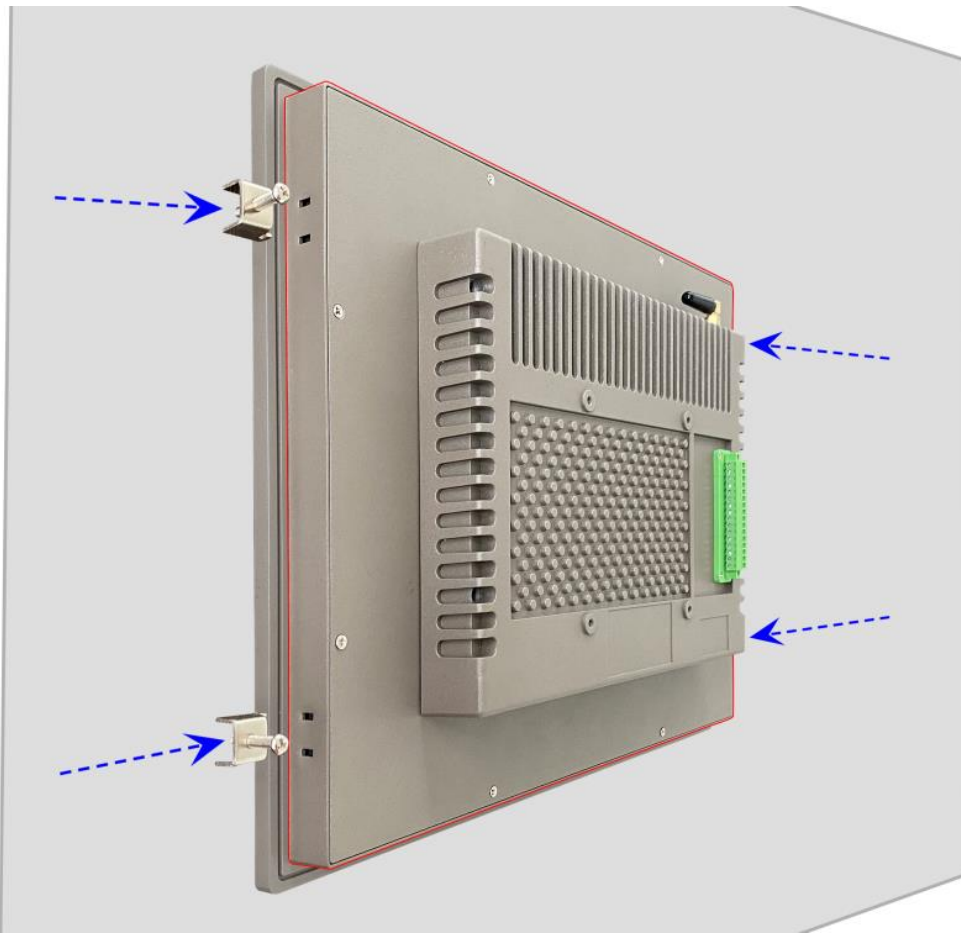
Figure 564: Panel Mounting-2
