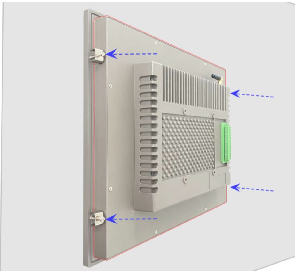
Figure 565: Panel Mounting-3
