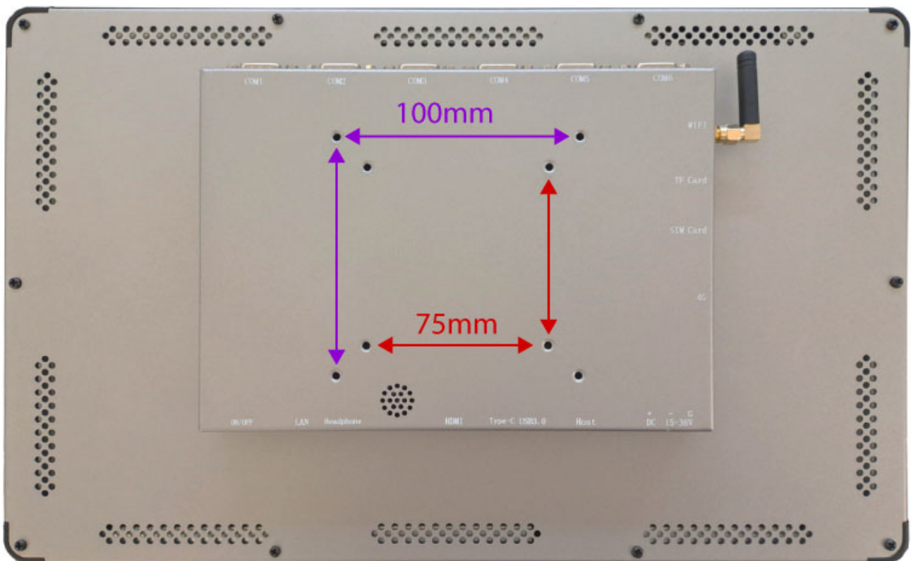
Figure 585: Mounting Method
