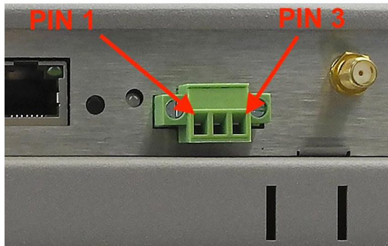
Power Input
