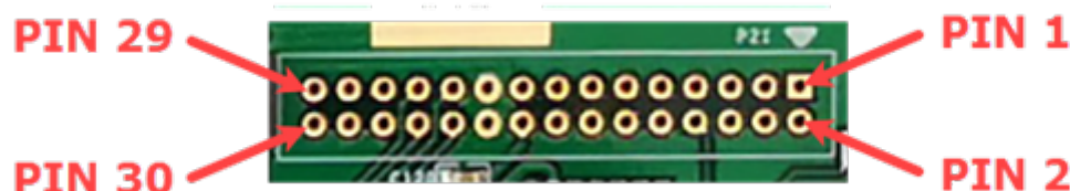
Figure 9: Expansion Port
