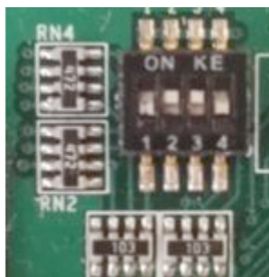
Figure 14: Boot DIP Switch
