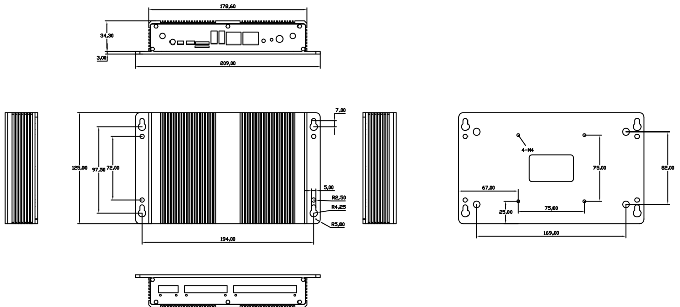
Figure 988: CS-CM4-BOX Technical Drawing
