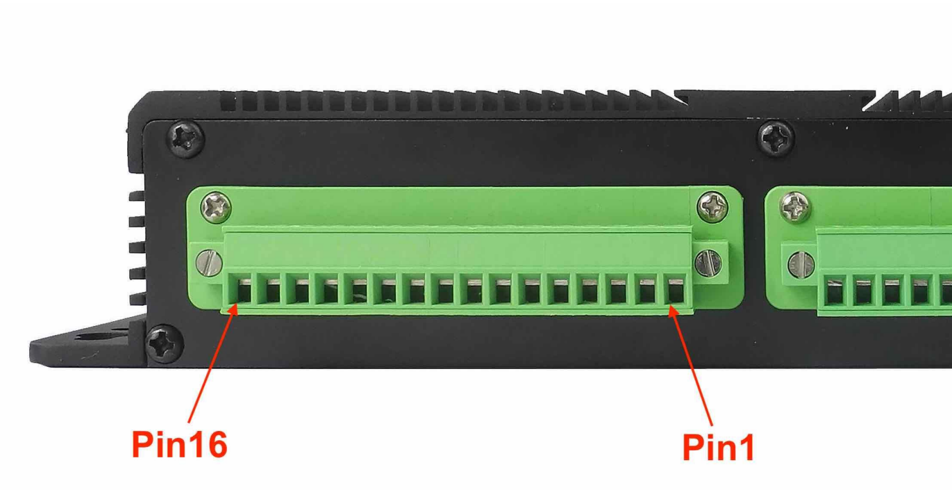
RS232-RS485-CAN on the CS-CM4-BOX Industrial PC
