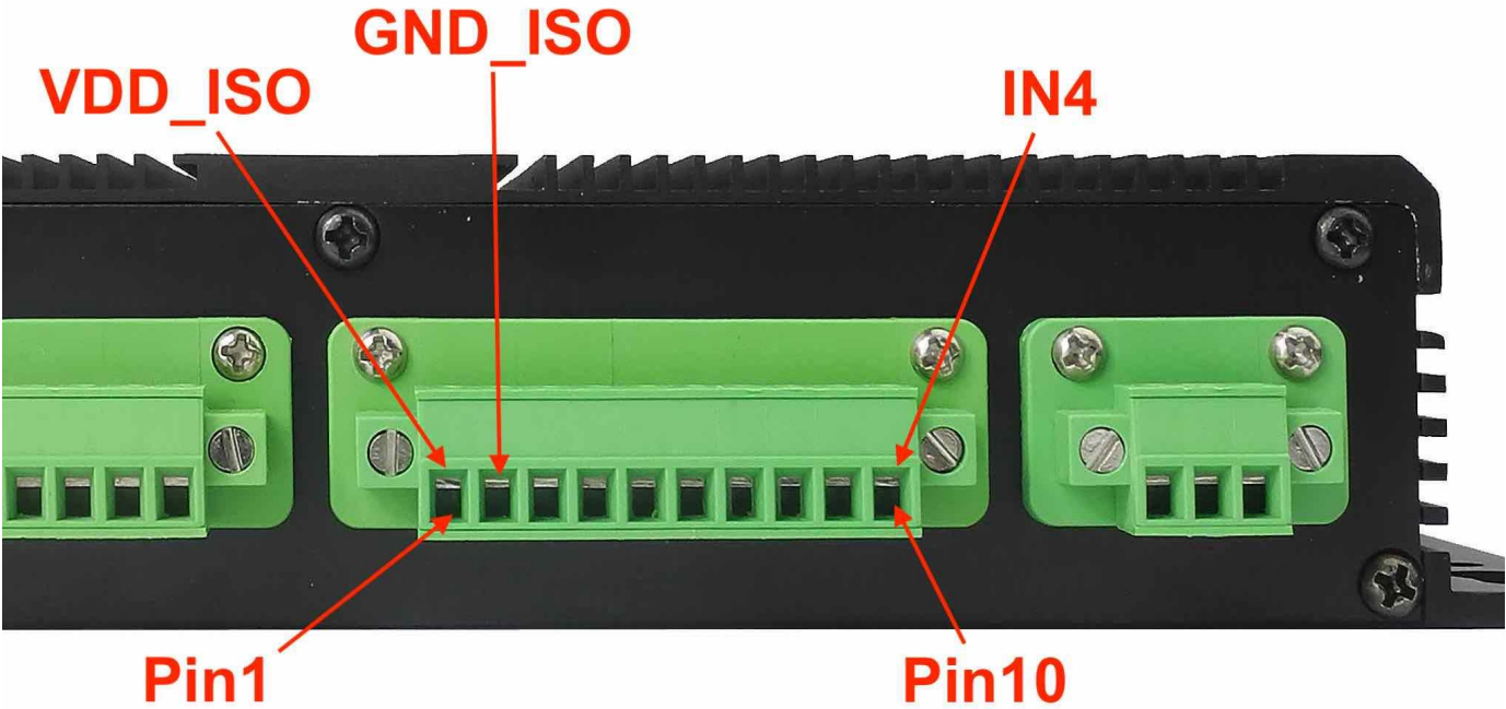
GPIO Connector
