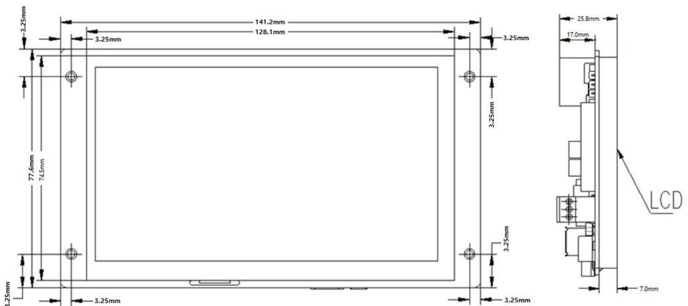
Figure 943: CS12720RA4050E Technical Drawing
