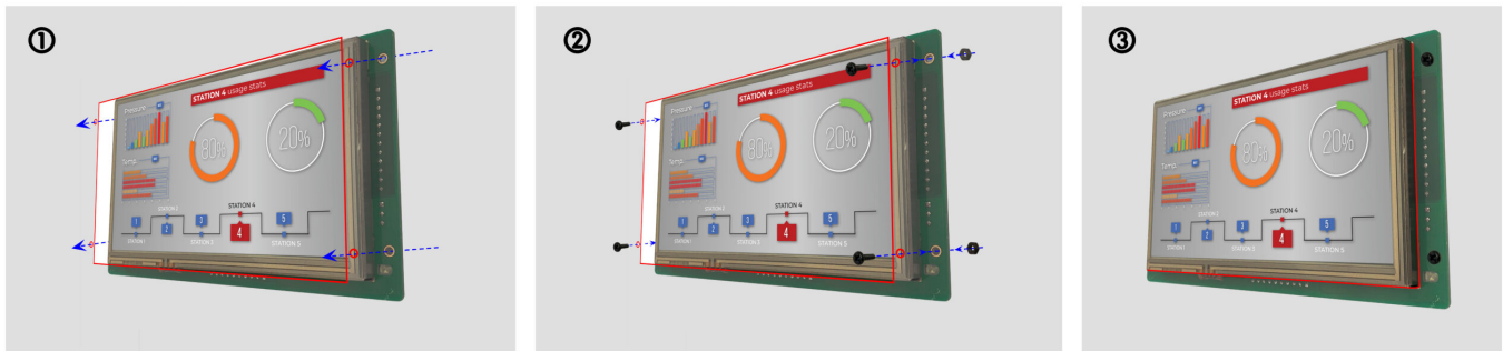
Figure 942: Embedded mounting
