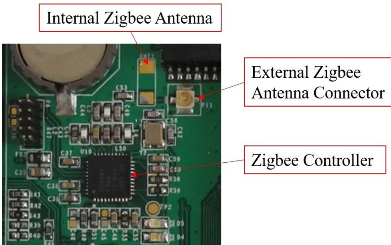
Figure 949: Zigbee controller
