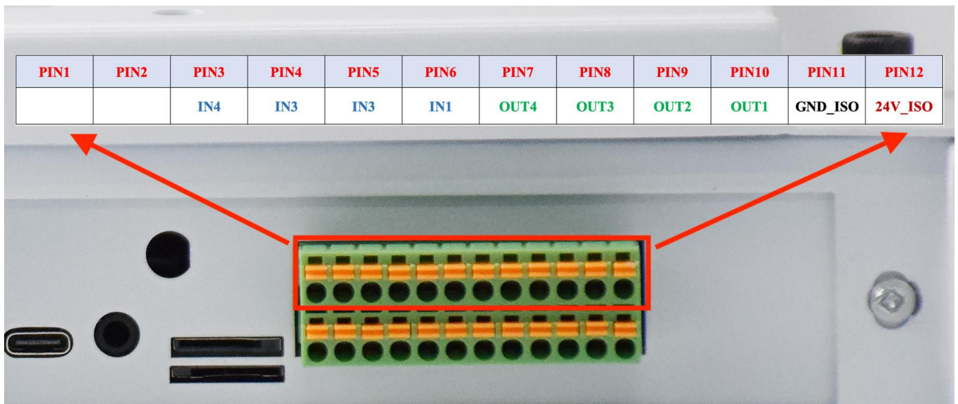
GPIO Connector
