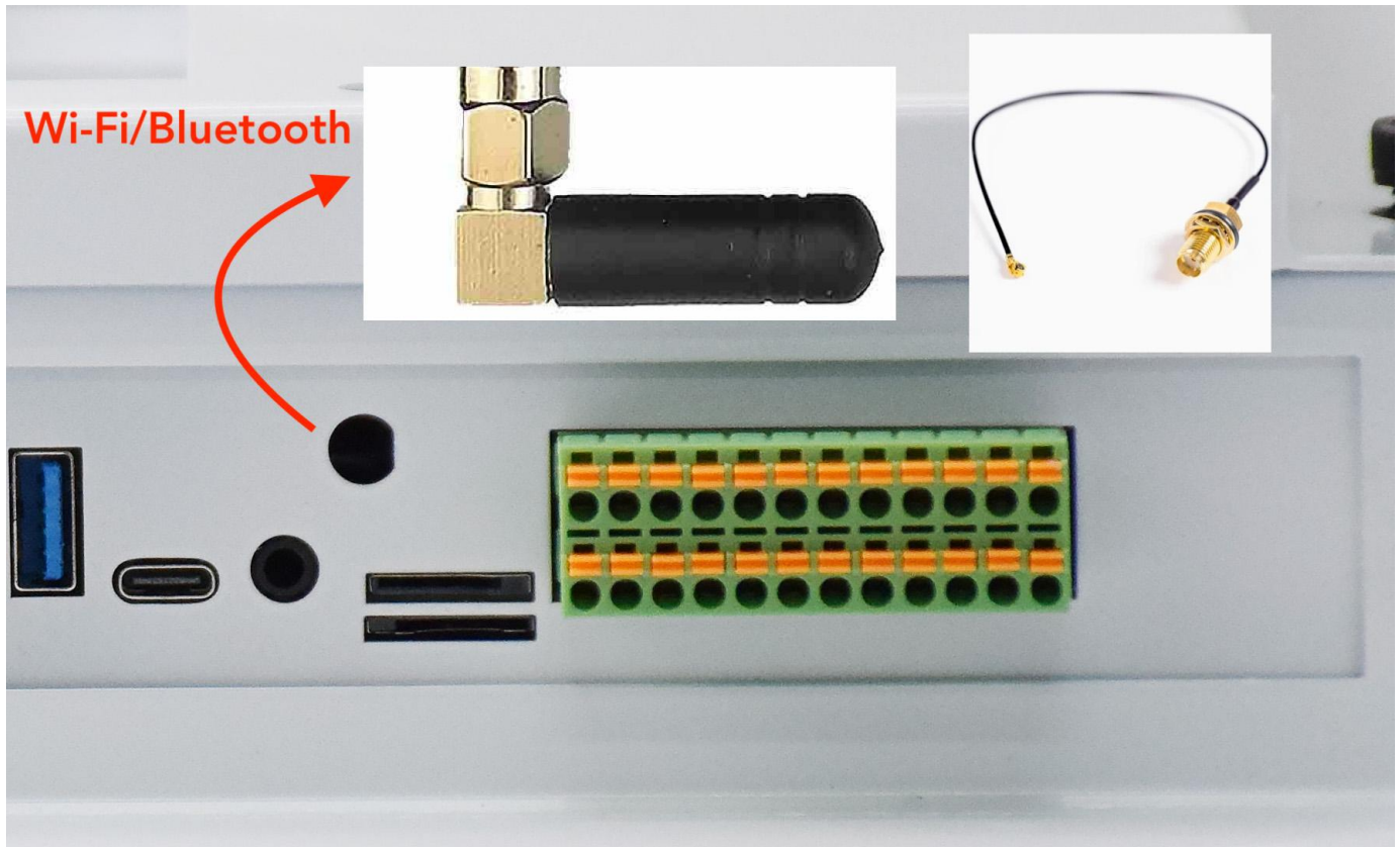
WiFi+BT Antenna
