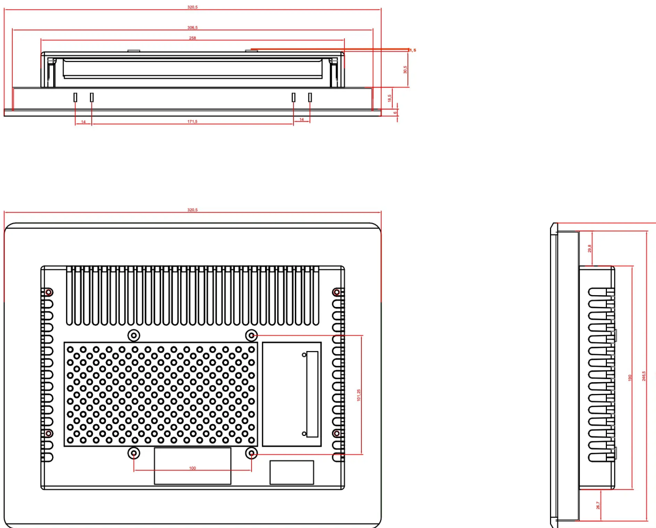
Figure 963: CS10768RA4121P Technical Drawing
