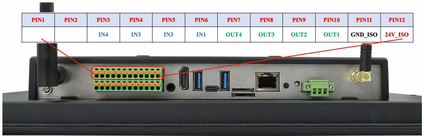
GPIO Connector
