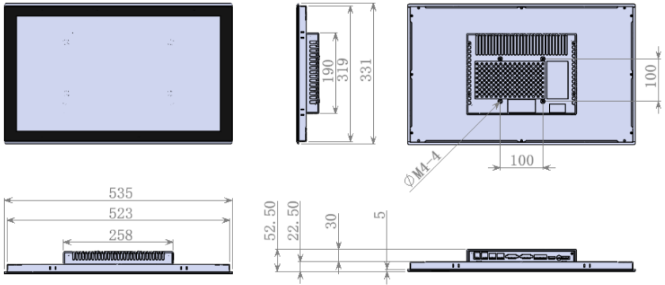
Technical Drawing
