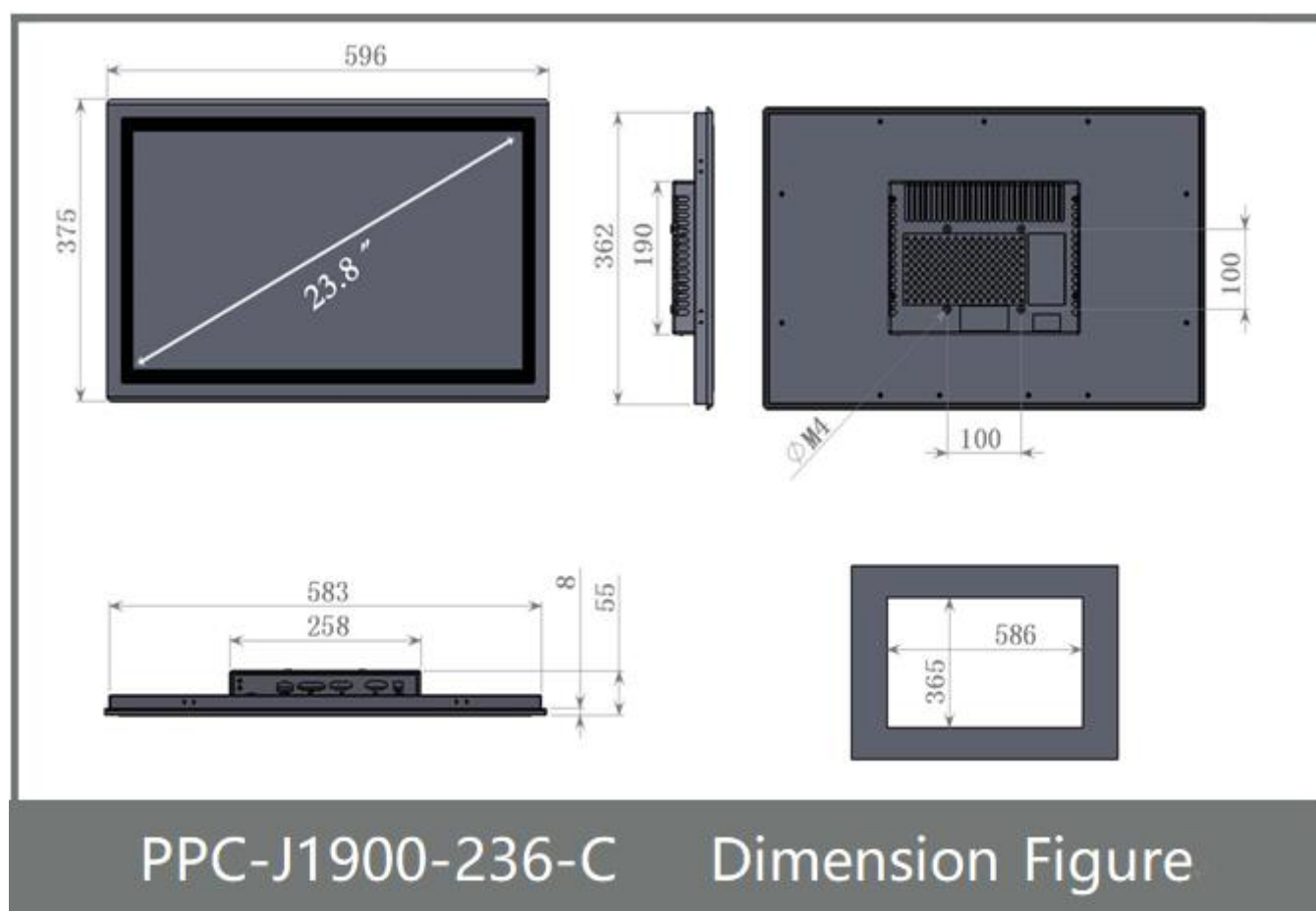
Figure 909: PPC-J1900-236-C Technical Drawing
