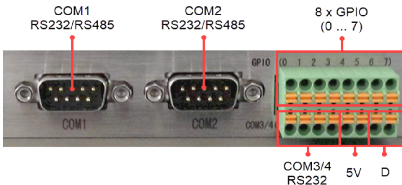
Figure 905: Figure 2: Connectivity Section - 2 x D-sub Connectors & 16-pin Double-Row Pluggable Terminal Block
